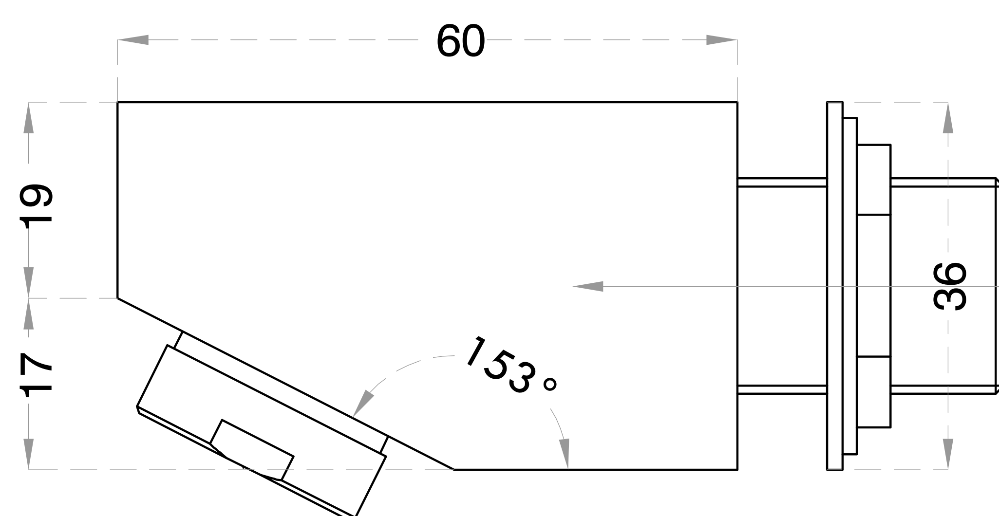
SIDE ELEVATION
