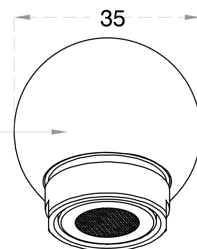
FRONT ELEVATION
